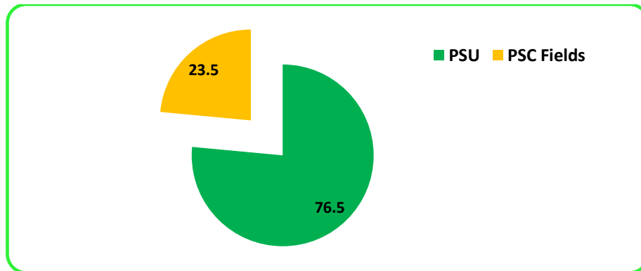
Figure-1; Percentage share in crude oil and condensate production; April 2024 (P)
