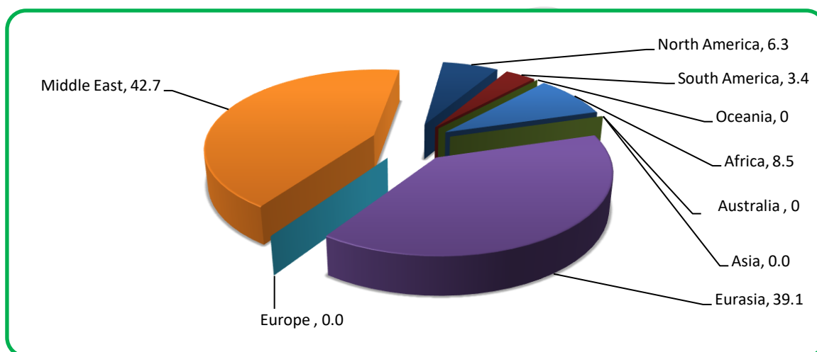
Figure 7: Region wise percentage share (%) of crude oil during April 2024 (P)
