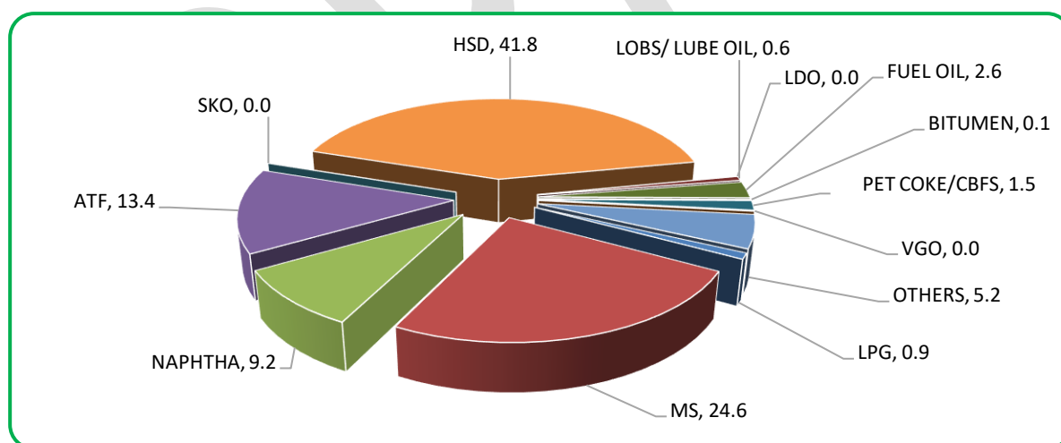
Figure 9: Percentage share of petroleum products in export: April 2024 (P)
