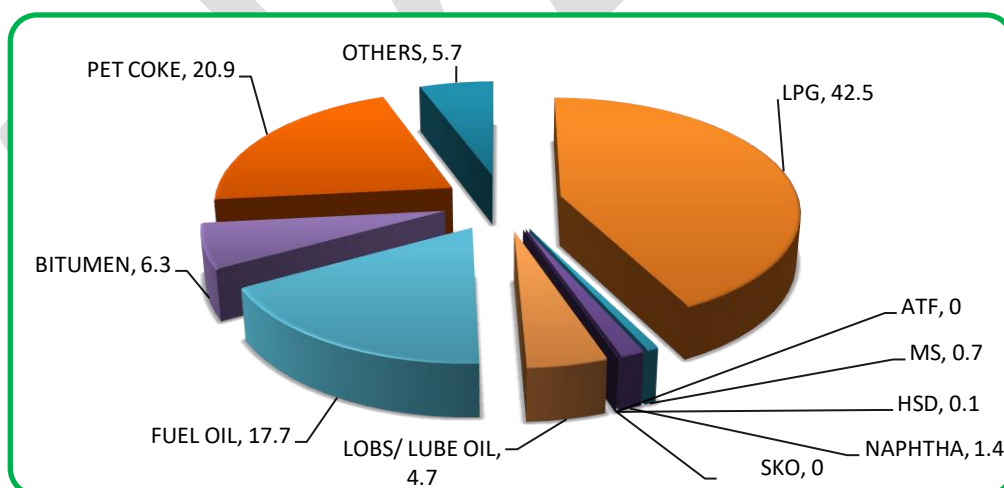
Figure 8: Percentage share of petroleum products in imports: April 2024 (P)
