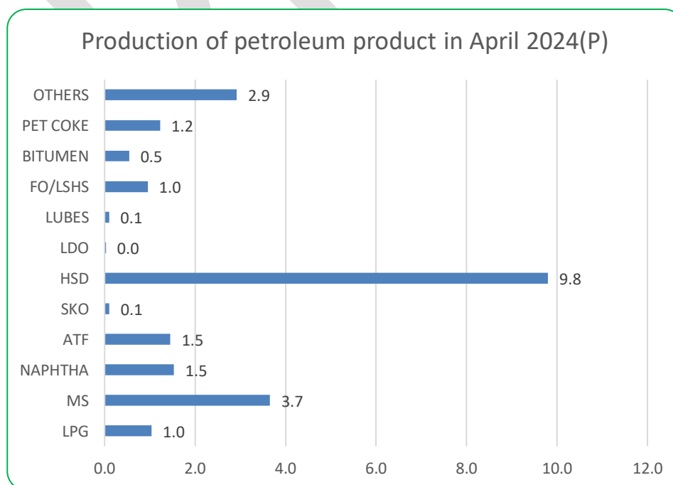
Figure-5; Product wise production of POL products by refineries and fractionators: April 2024 (P)
