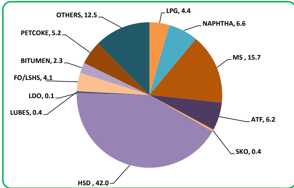
Figure-6; Percentage share of products in total POL production: April 2024 (P)
