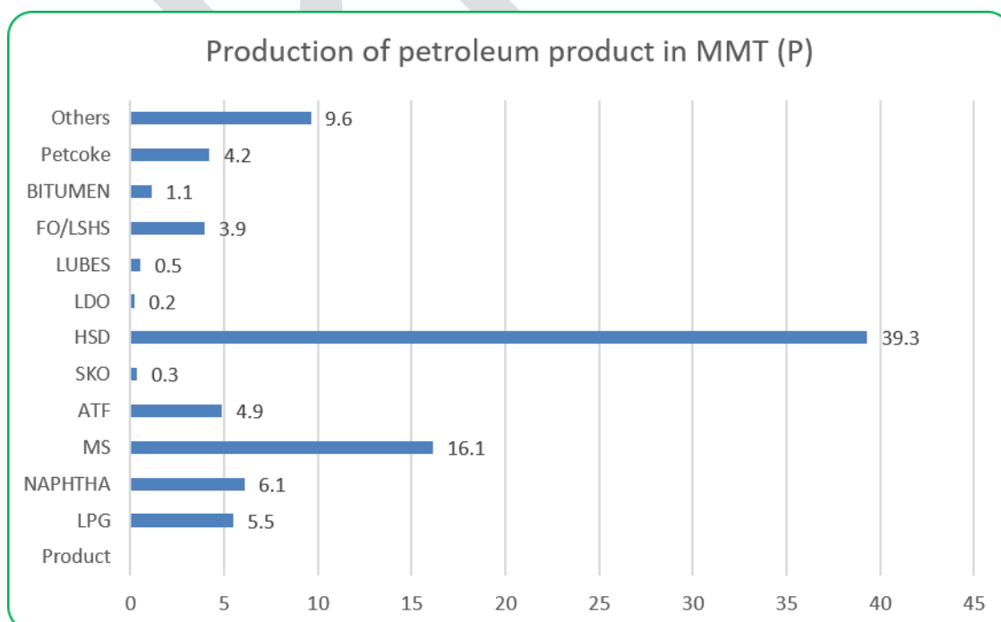
Figure-5; Product wise production of POL products by refineries and fractionators: April- July FY 2026-27 (P) (P)
